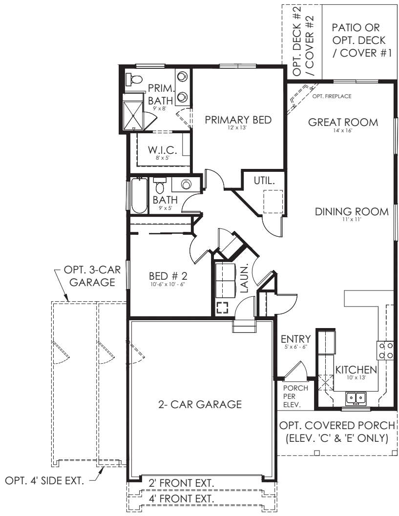
MAIN LEVEL 1,379 SF
